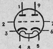
Noval B9A
